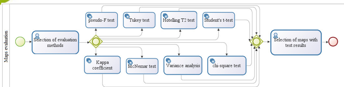
Figure 6. Reference process for maps evaluation modelled in BPMN.
